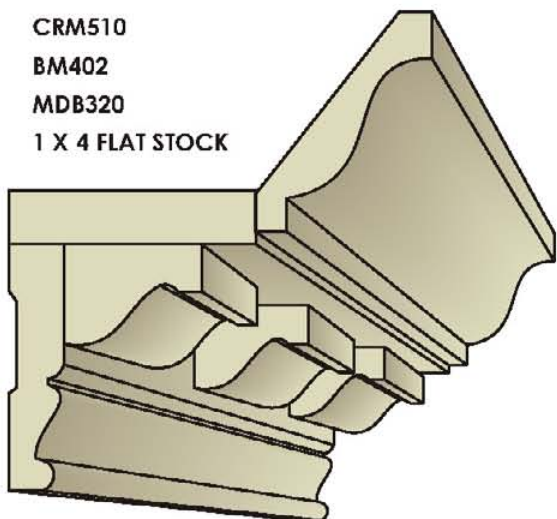
BUILT-UP CORNICE WITH MODILLION BLOCKS
