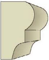
PNM201 5/8" X 1"
